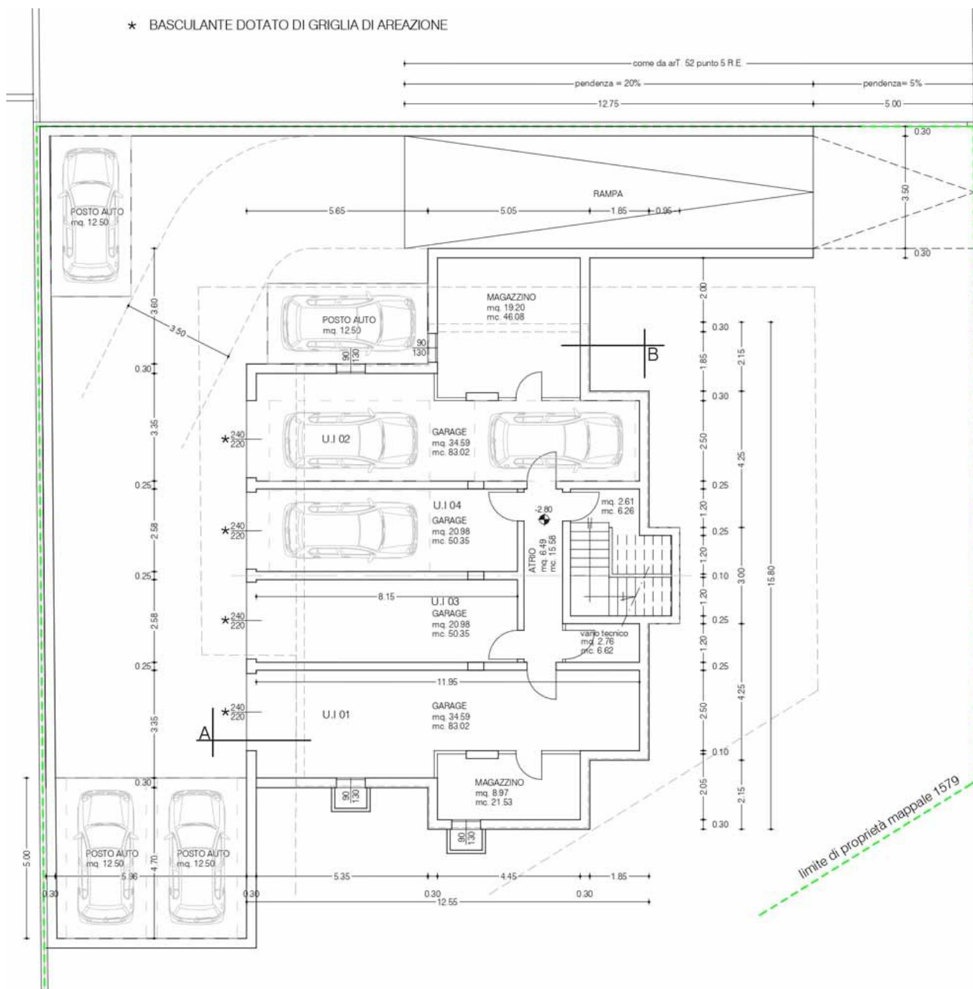
PIANO INTERRATO
